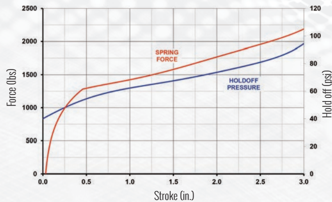
30RPC3 (30SCL3R) Chamber Performance
